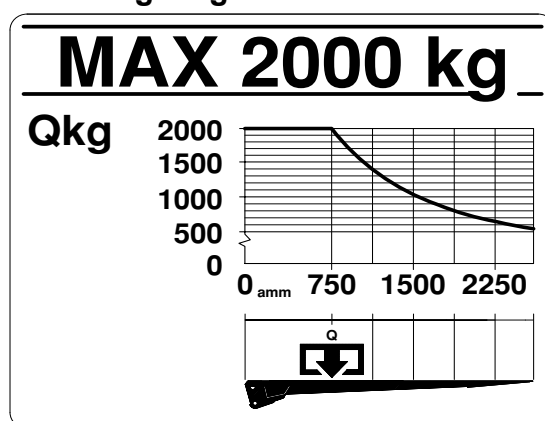
Loading diagram
