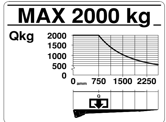
Loading diagram
