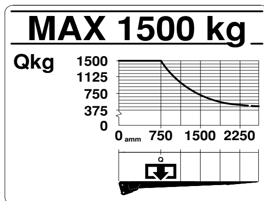
Loading diagram
