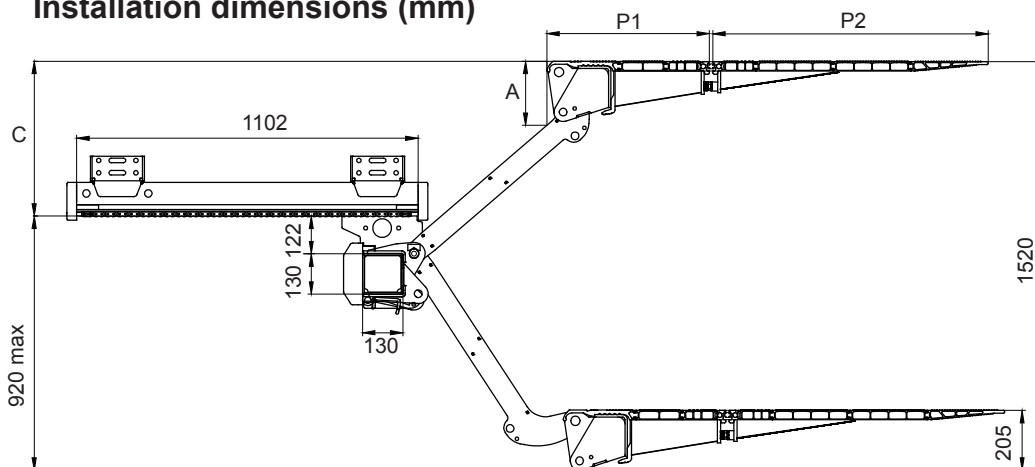
Single folding platform
