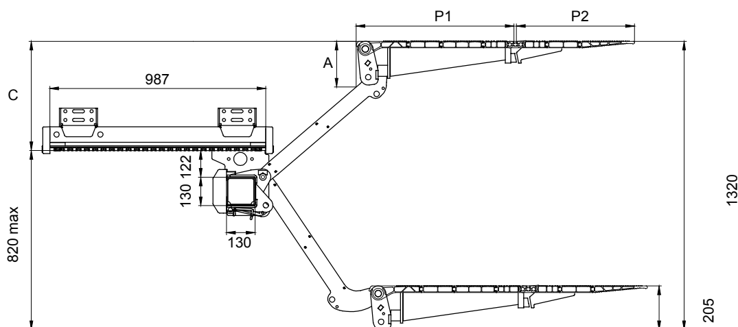
Installation dimensions (mm)
