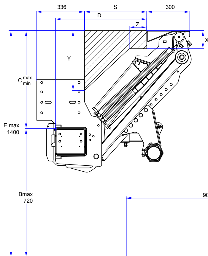
Installation dimensions (mm)
