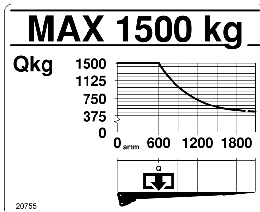
Loading diagram
