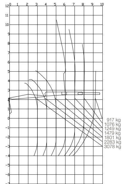
Load diagram F96S 97 HPL
