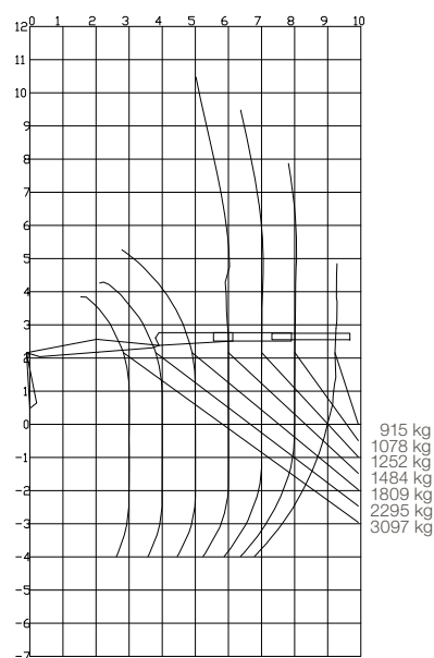
Load diagram F96S 97
