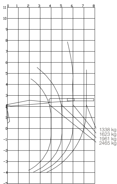
Load diagram F96S 79 HPL
