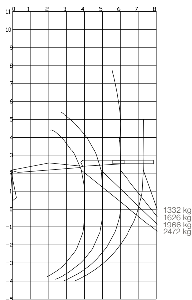
Load diagram F96S 78
