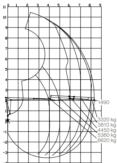
Load diagram F281S83
