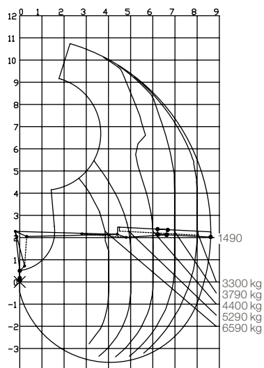
Load diagram F281S86
