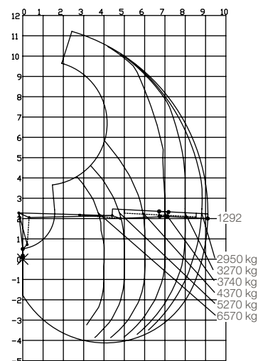
Load diagram F281S91
