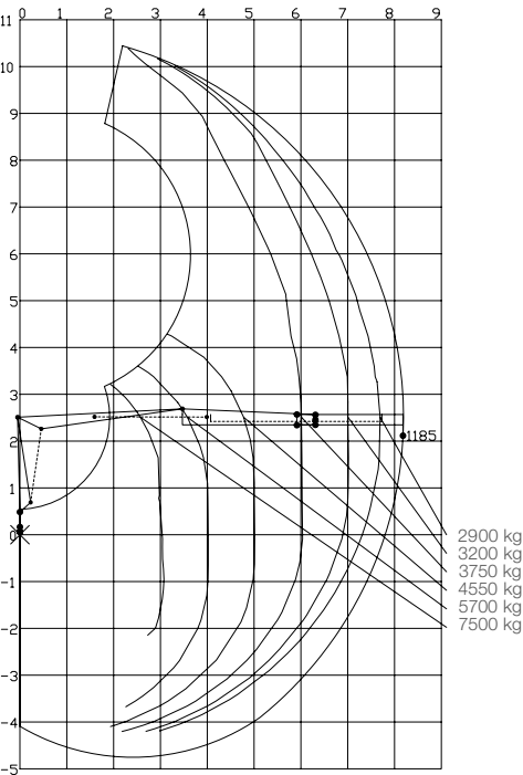
Load diagram F265Z 82
