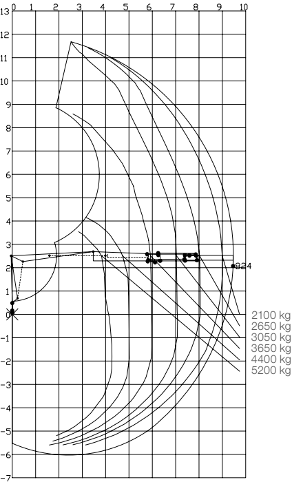
Load diagram F265Z 82 Booster
