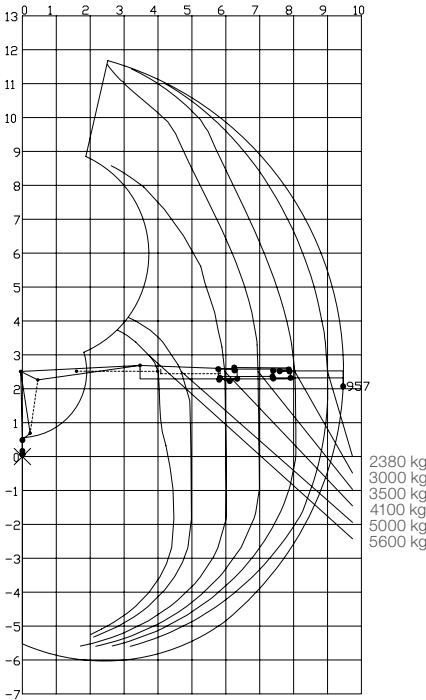
Load diagram F265Z 95 Booster
