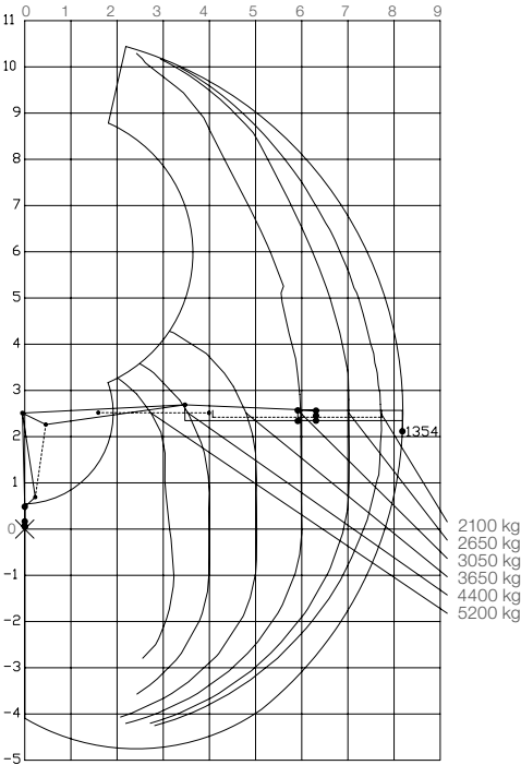
Load diagram F265Z 95
