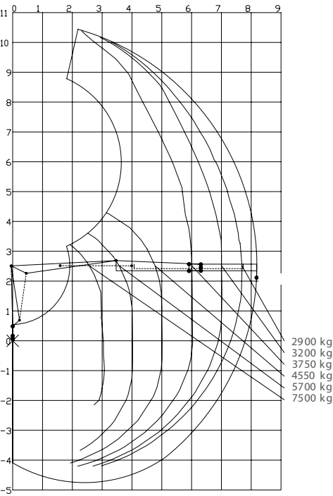
Load diagram J2640Z 82
