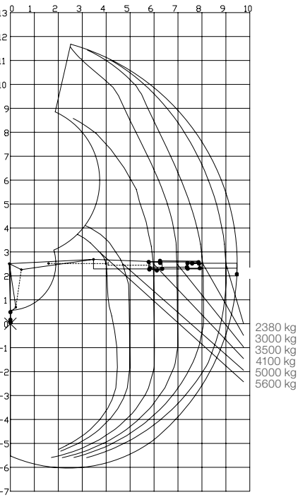
Load diagram J2640Z 95 Booster
