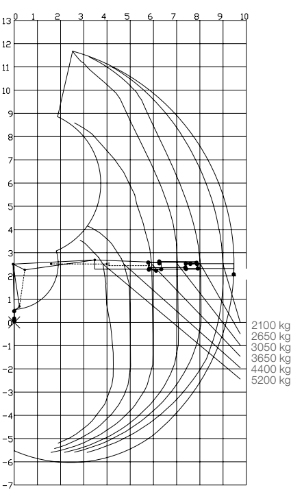
Load diagram J2640Z 95
