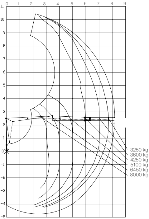
Load diagram J2640Z 82 Booster
