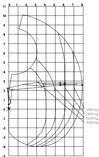
Load diagram J1420S 79 BOOSTER
