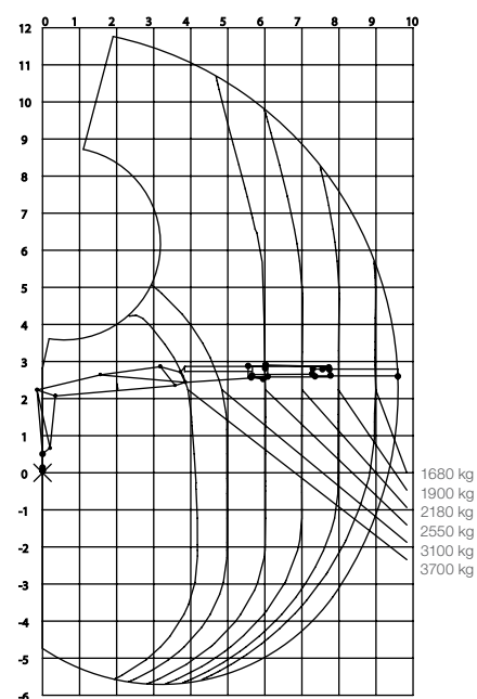
Load diagram J1420S 96i BOOSTER
