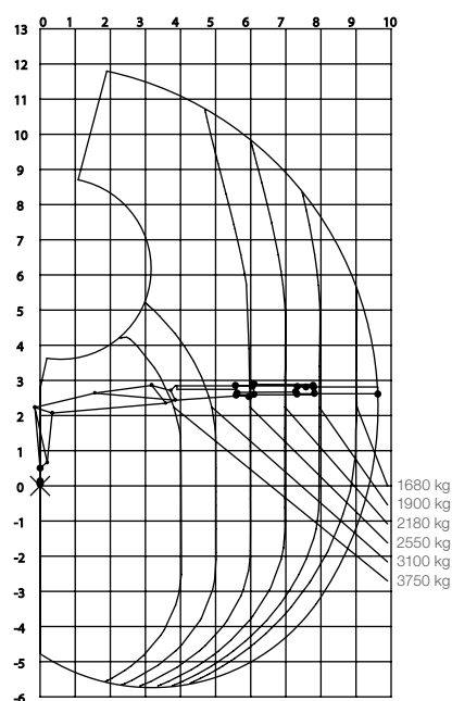
Load diagram J1420S 96 BOOSTER
