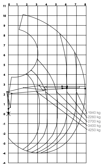
Load diagram J1420S 79
