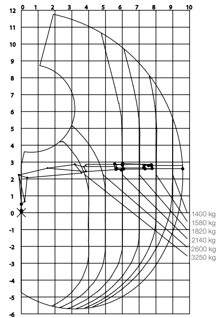
Load diagram J1420S 96i
