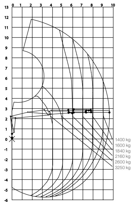
Load diagram J1420S 96
