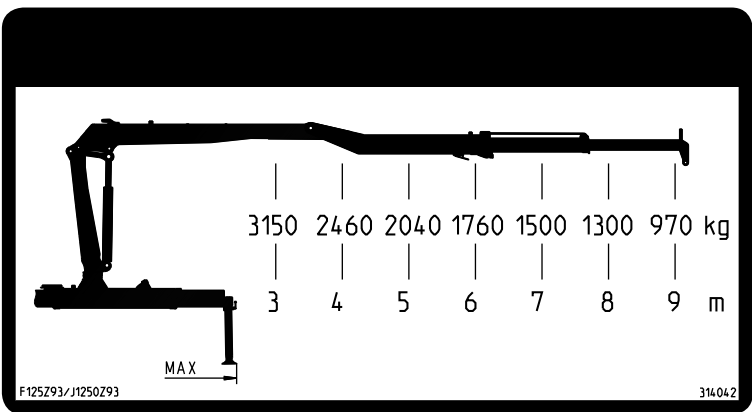
Load chart 1250Z93
