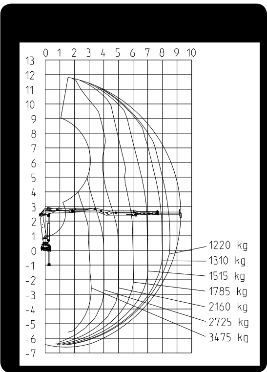
Load diagram 1250Z93
