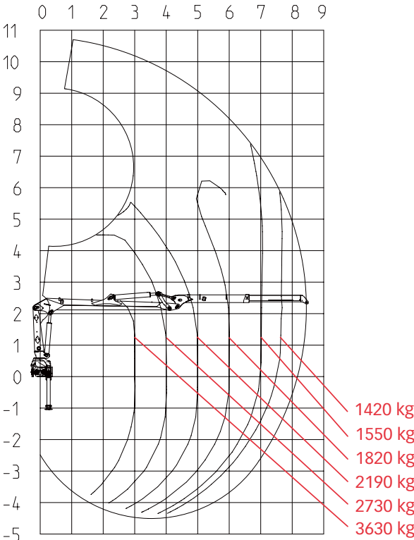
Load diagram JONSERED 1088S84i
