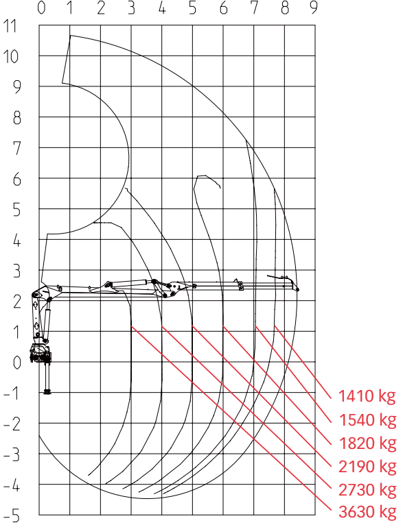
Load diagram JONSERED 1088S84
