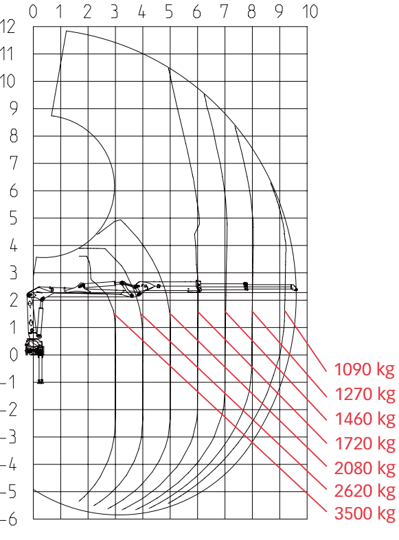
Load diagram JONSERED 1088S96i
