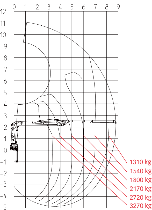
Load diagram JONSERED 1088S88i
