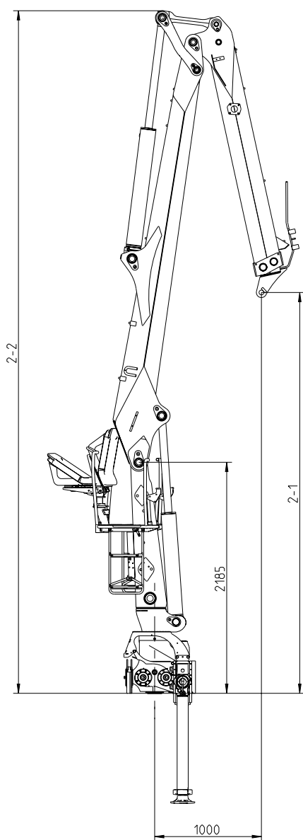
Upright view with top seat
