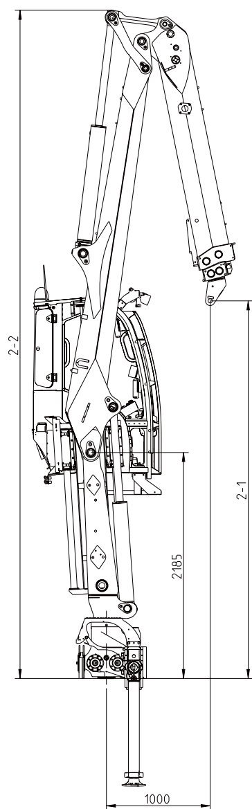
Upright view with cabin C912
