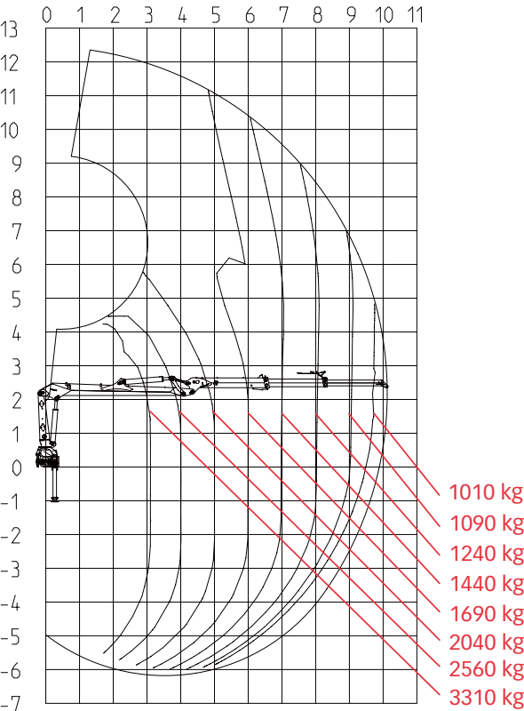
Load diagram JONSERED 1088S101
