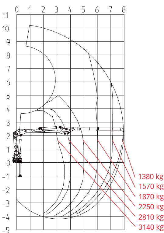
Load diagram JONSERED 1088S79i
