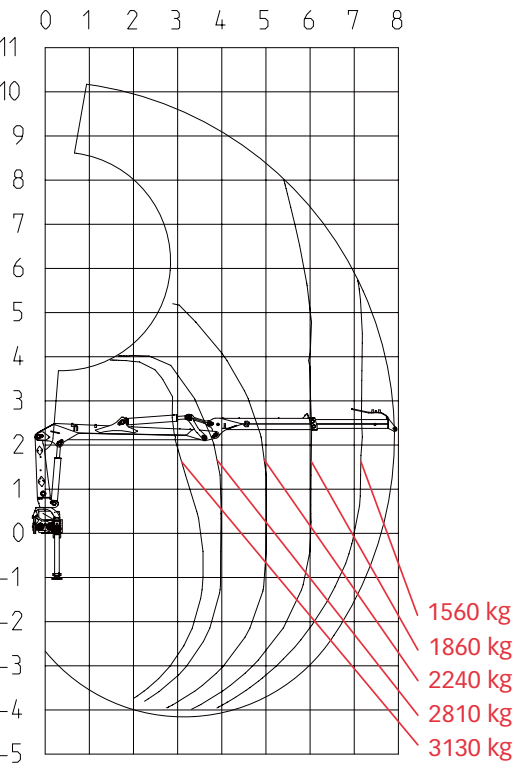
Load diagram JONSERED 1088S79
