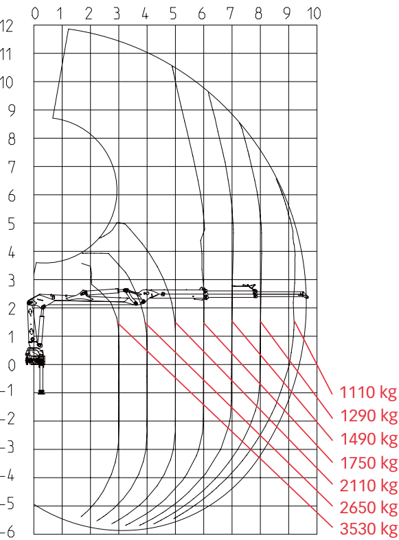
Load diagram JONSERED 1088S96
