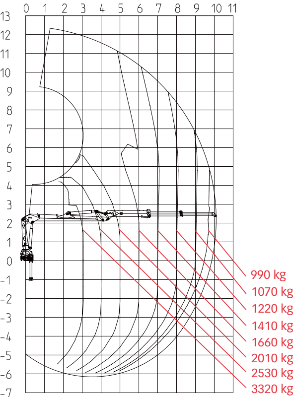
Load diagram JONSERED 1088S101i
