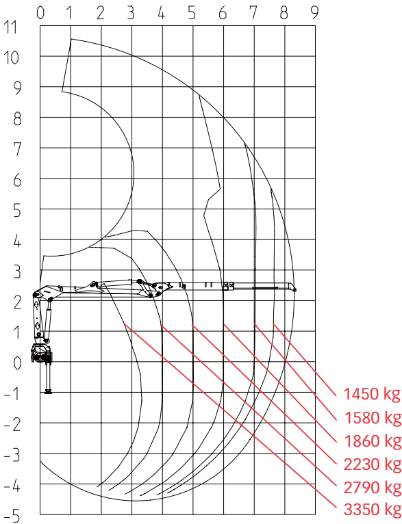
Load diagram JONSERED 1088S83i
